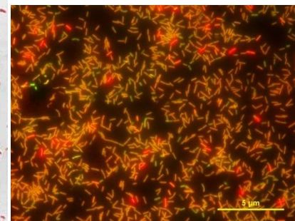
Fluorescence microscopy
